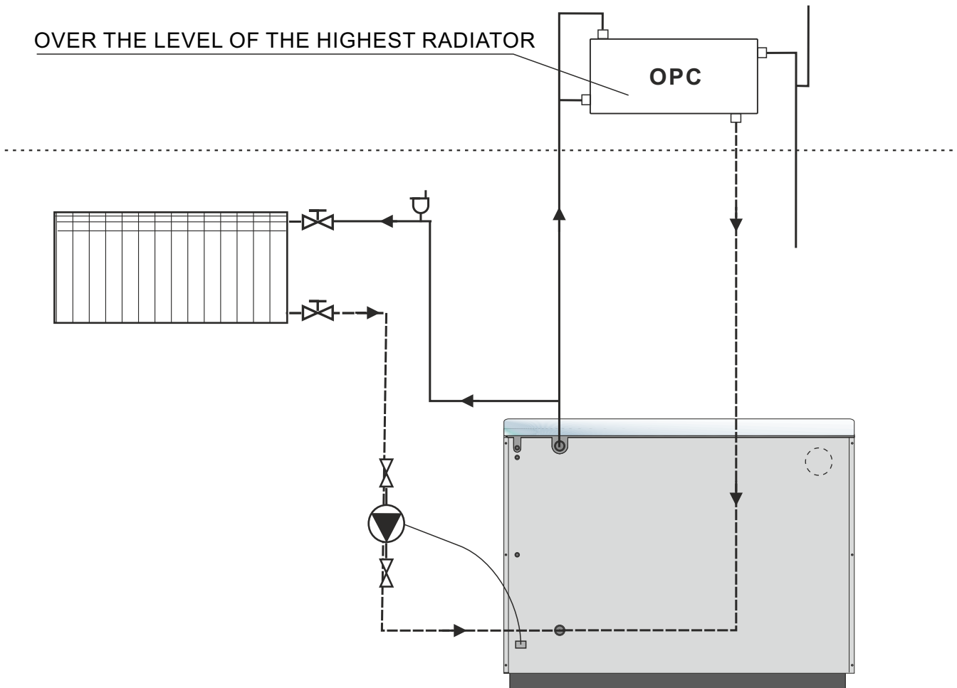
Scheme 1. Connecting an BIO-PEK B - L (applies to BIO-PEK B - D)
