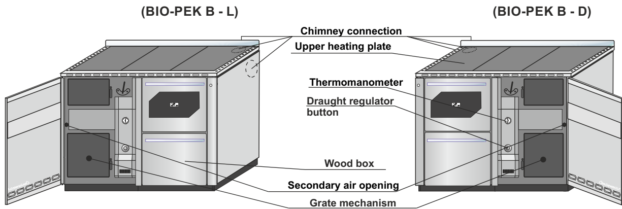
Image 9. Basic parts
